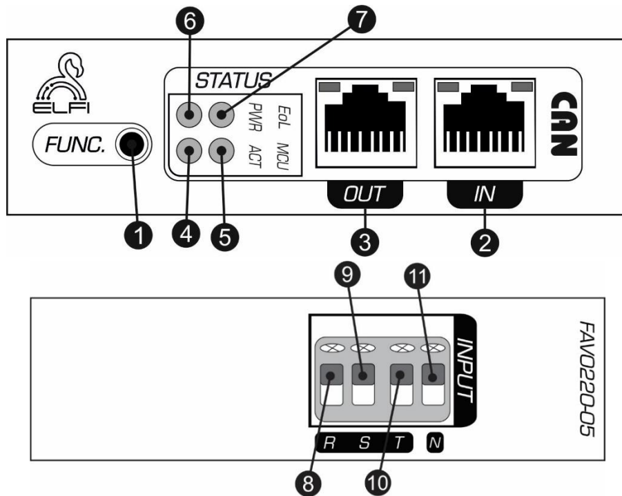
Figure 2: Side view of a 3-Channel AC Voltage Detector Node
