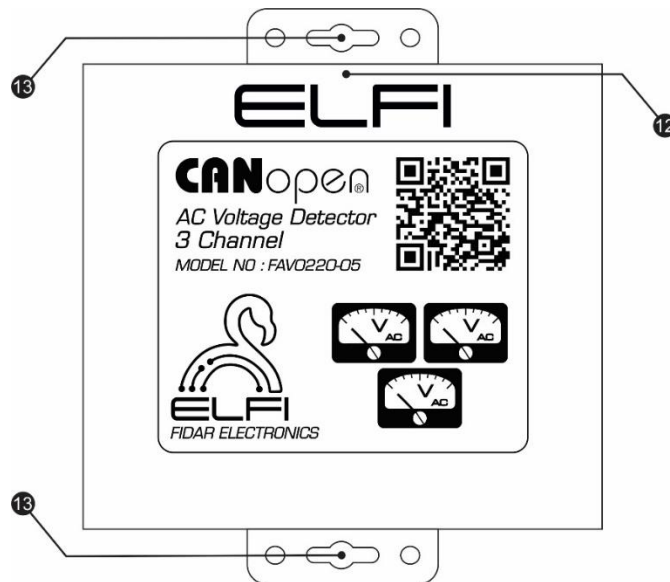
Figure 3: Front view of a 3-Channel AC Voltage Detector Node
