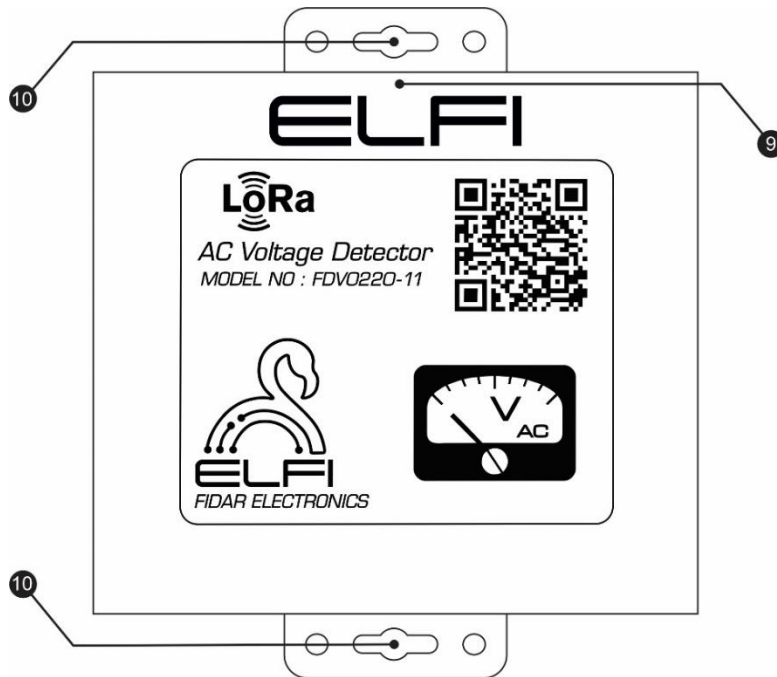
Figure 3: Front view of a Wireless Single-Channel AC Voltage Detector Node
