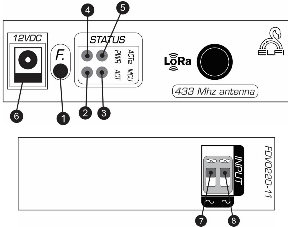
Figure 2: Side view of a Wireless Single-Channel AC Voltage Detector Node
