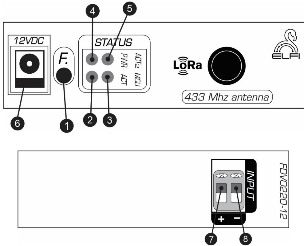
Figure 2: Side view of a Wireless Single-Channel DC Voltage Detector Node
