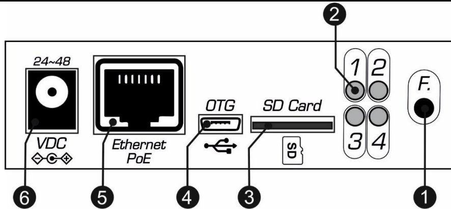
Figure 2: Side view the detector
