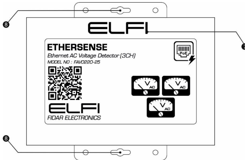
Figure 3: Front view of the detector
